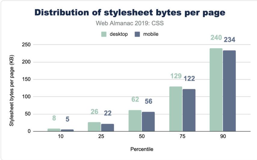
Figure 2.35. Distribution of the number of stylesheet bytes (KB) loaded per page.
