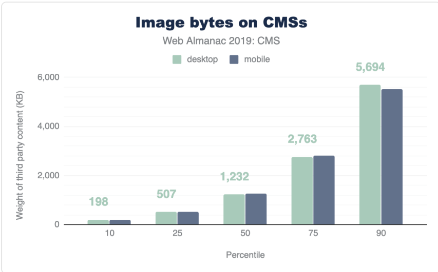
Figure 14.12. Distribution of image weight (KB) on CMS pages.
