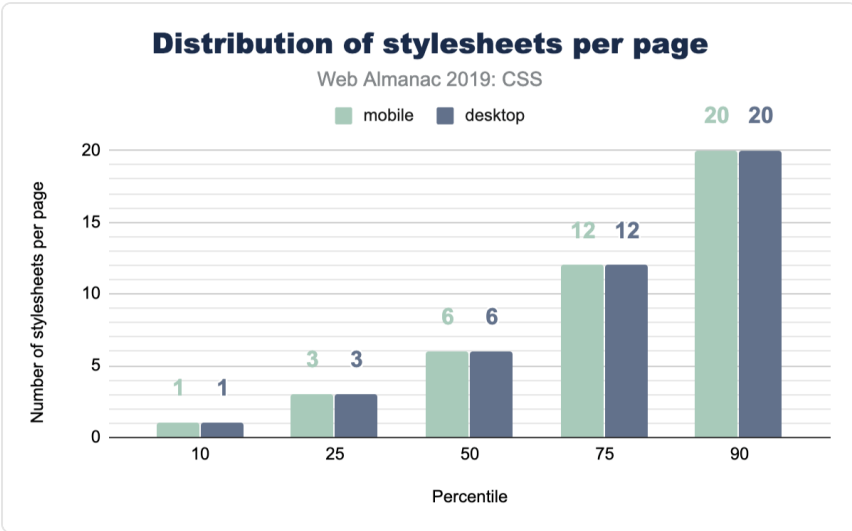
Figure 2.33. Distribution of the number of stylesheets loaded per page.
