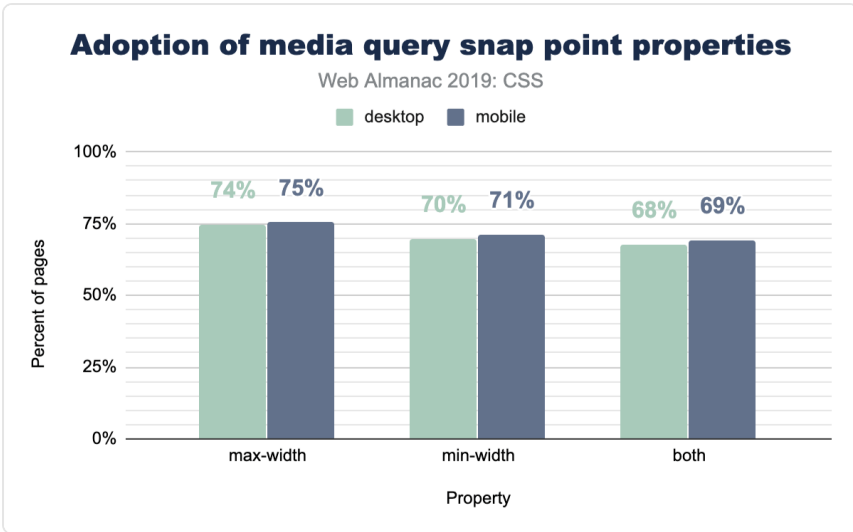
Figure 2.31. Adoption of properties used in media query snap points.
